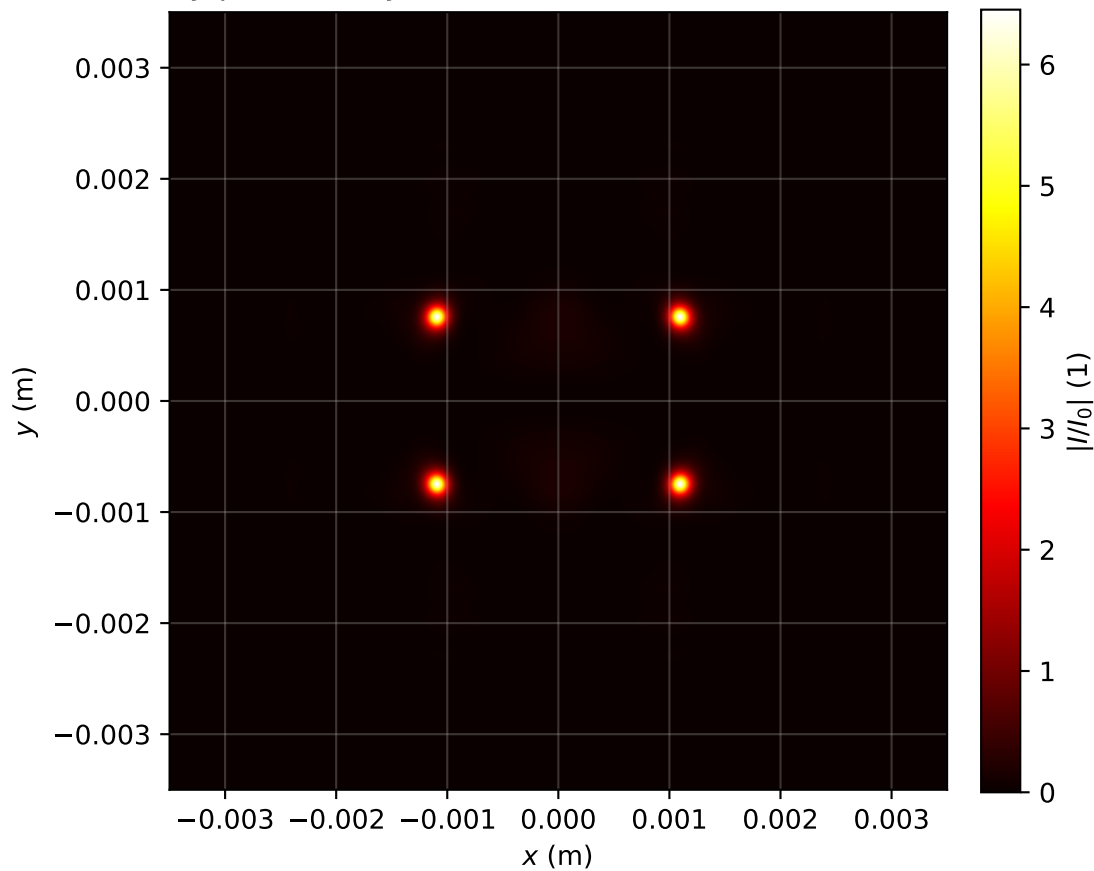
Intensity profile I(x, y, z = 2.627)/I_0 , P_{in}=7.0P_{cr} , artificial time
